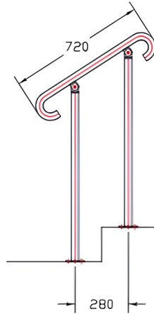
1-Step Freestanding
